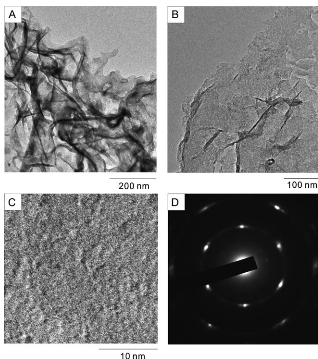
Figure 4. A–C) TEM images of large graphene sheets at different magnifications. D) Electron diffraction pattern of the graphene sheet in (B).
